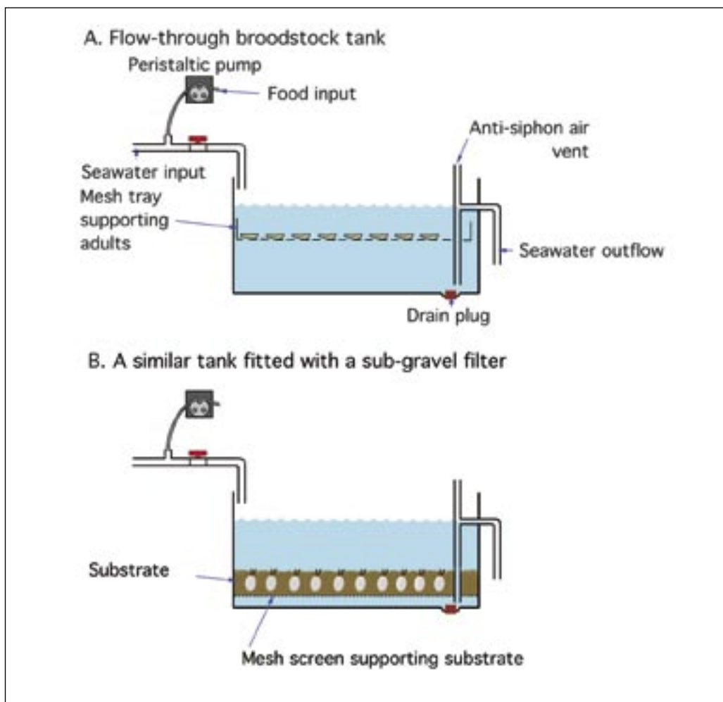
Figure 35: Diagrammatic representation of A – a flow-through broodstock tank in which adults are suspended off the bottom in a mesh tray with large apertures in the base so as not to retain faeces and detritus; B – a similar tank fitted for sub-gravel filtration. Systems of type A are suitable for most species that do not require a substrate. Clams and some scallop species often condition better in tanks of type B.
